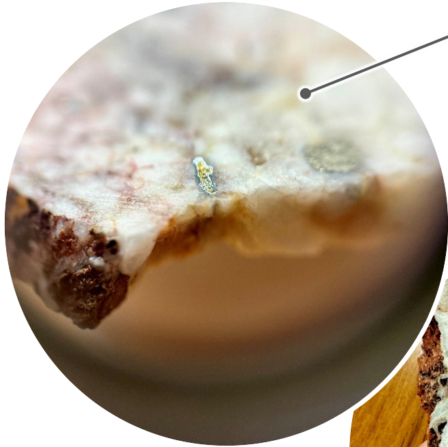
Copper sulphide bearing quartz vein, Loki (Champion, NT)
